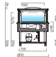
IFDT 800 3M1-3L1 dual-temperatura dual-temperature dual-température dual-temperatura
